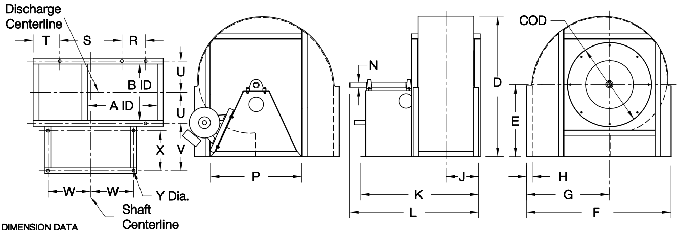
DIMENSION DATA
