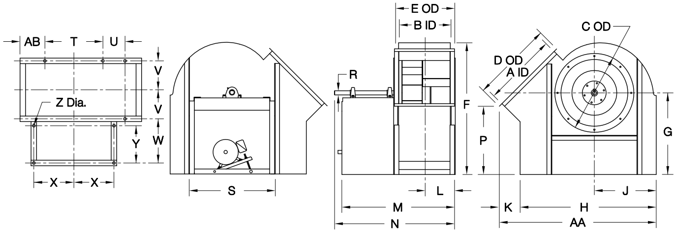
DIMENSION DATA
