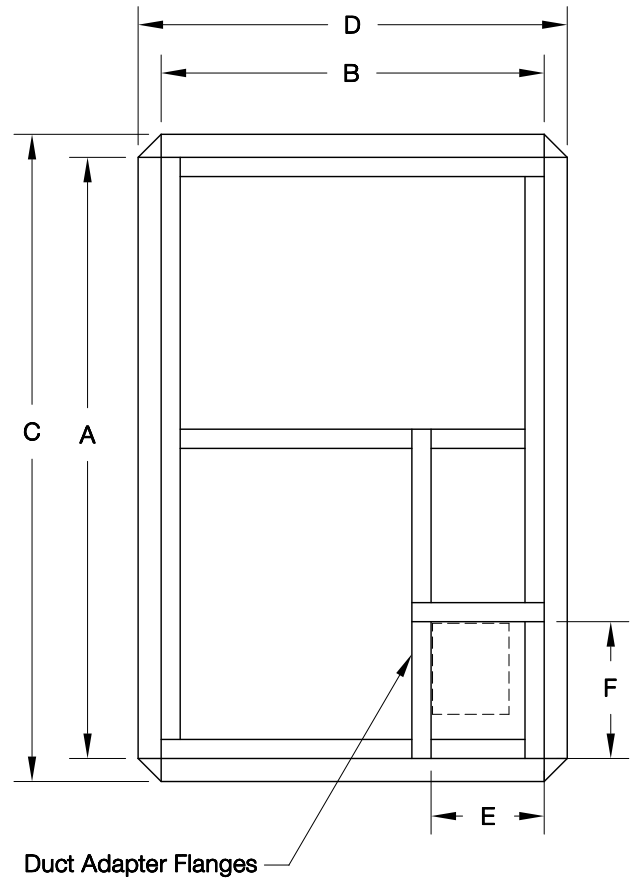
ERV CURB TOP VIEW ARR. C SIZE 7000-10000
