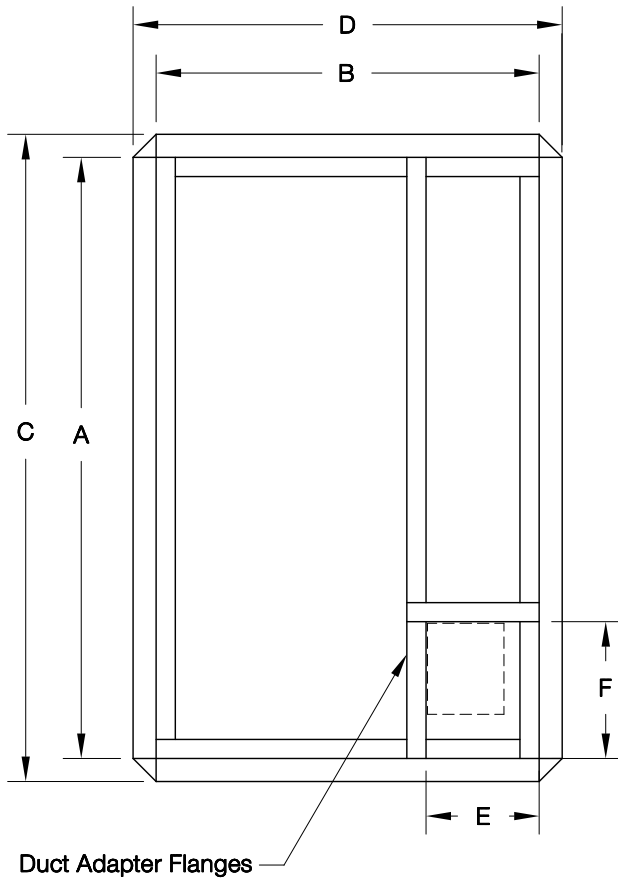
ERV CURB TOP VIEW ARR. C SIZE 1500-5500
