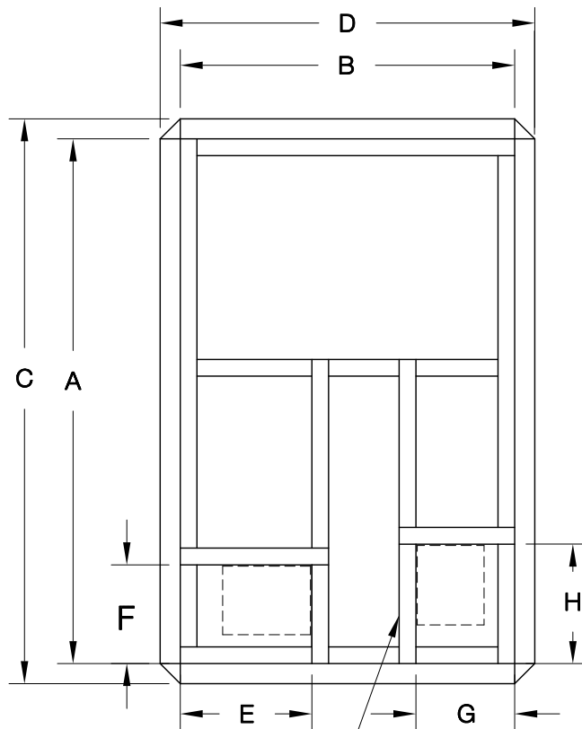
ERV CURB TOP VIEW ARR. V SIZE 7000-10000
