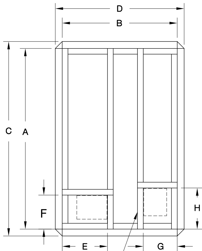
ERV CURB TOP VIEW ARR. V SIZE 1500-5500
