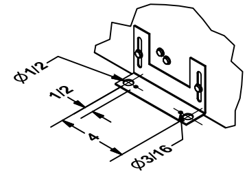
MOUNTING BRACKET DETAIL
