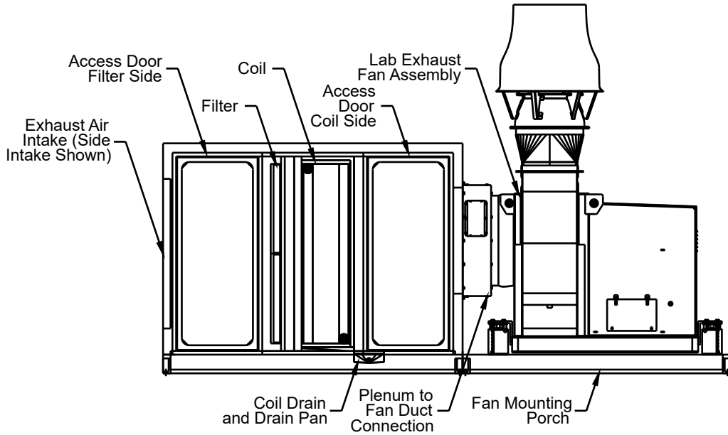
Standard Construction
