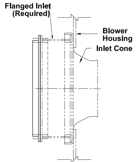
FLANGED INLET WITH COMPANION FLANGE
