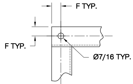
HOLE PATTERN DETAIL
